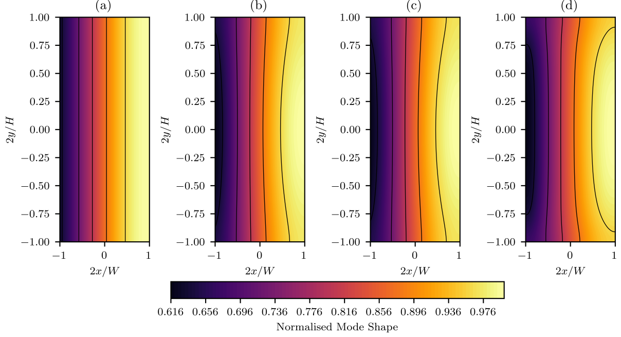
Fig. 7 Least attenuated modes obtained for upstream propagation with the reference impedance at 3000 Hz. (a) CHE+IMBC; (b) law-of-the-wall; (c) CFD, and; (d) hyperbolic tangent.
