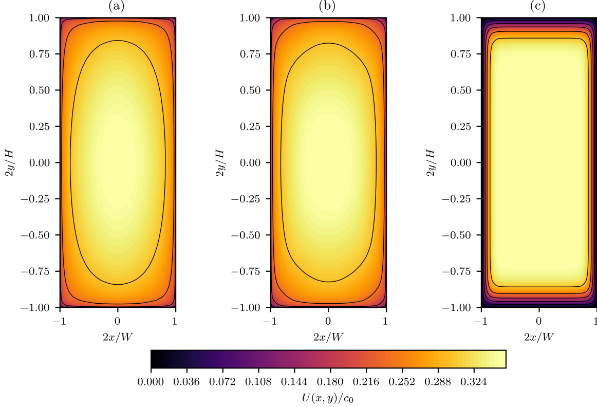
Fig. 2 Flow profiles considered in this work. (a) Tensorized law of the wall; (b) CFD evaluated, and; (c) tensorized hyperbolic tangent. Isolines represent contour axial velocity.
